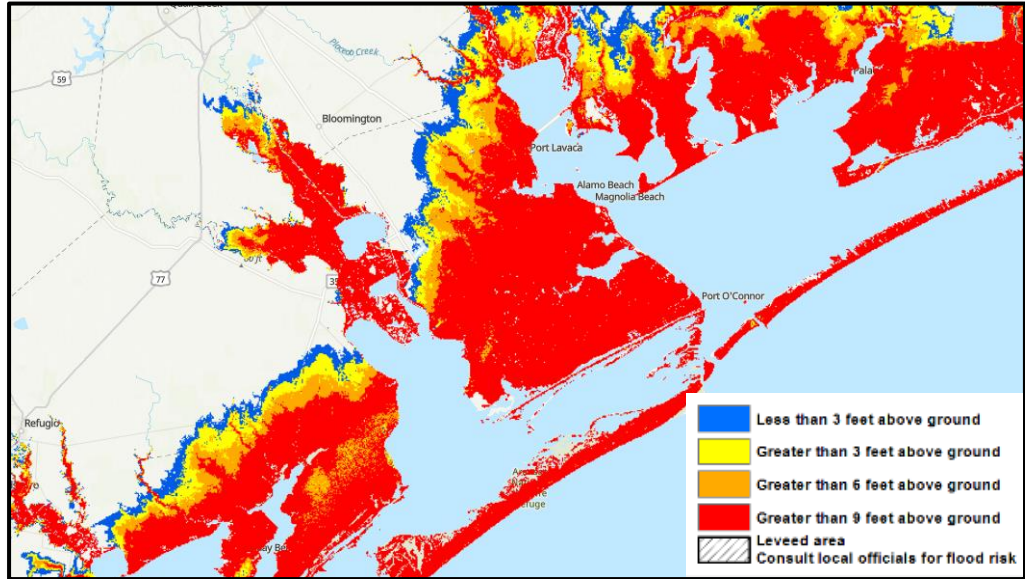
Above: This map shows the height above ground the water could reach and depicts the reasonable worst-case scenario from storm surge flooding.
